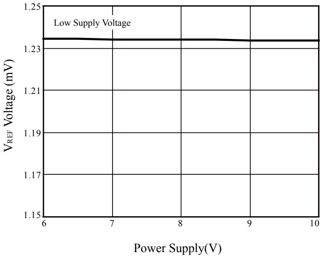
图8 V REF vs. Power Supply (Low Supply Voltage)
