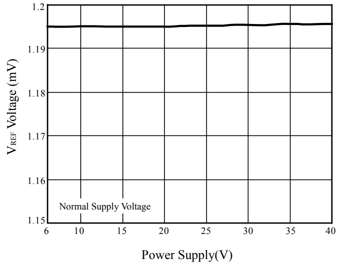
图9 V REF vs. Power Supply (Normal Supply Voltage)
